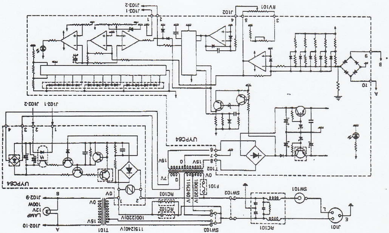
回路图: CIRCUI T DIAGRAM
